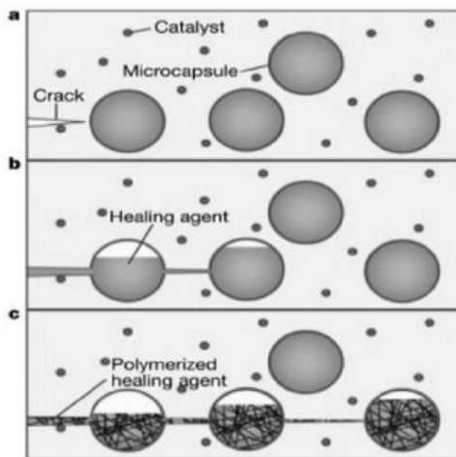
Mechanism of self healing concrete
