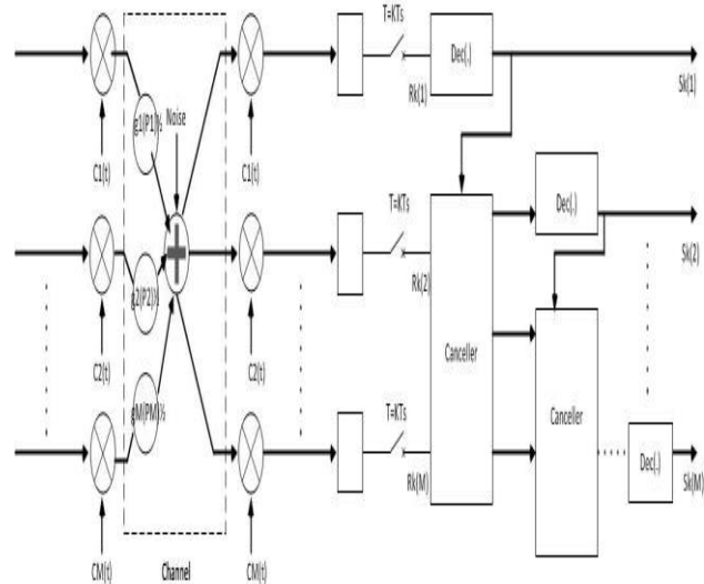
Fig.5 Multi User Detection (MUD) Receiver using Decision Feedback Mechanism[26][31][32]
