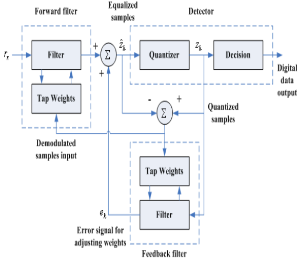
Fig.4 Decision Feedback (DFE) Equalization[32][33]
