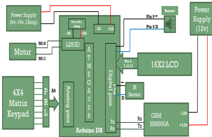
Fig. 11. Hardware Architecture
