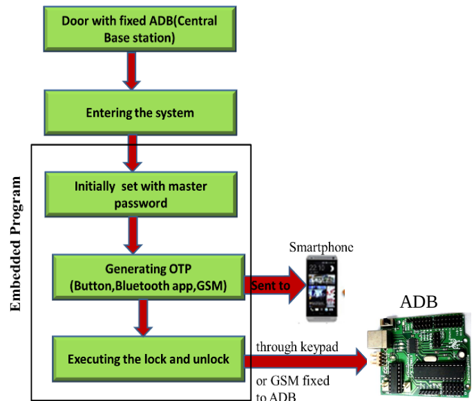
Fig. 10. Block Diagram
