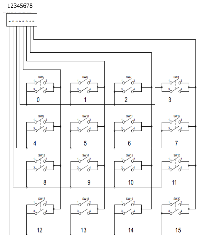
Fig. 8. Keypad Internal Connection
