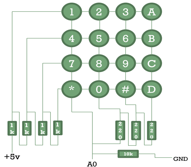
Fig. 12. Pin Reduction Logic
