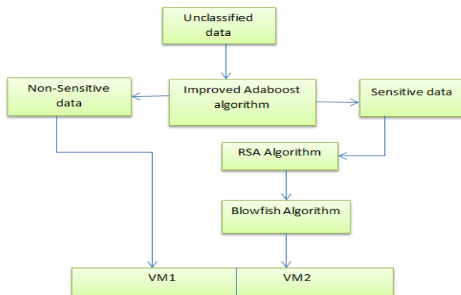
Figure 3: Proposed model
