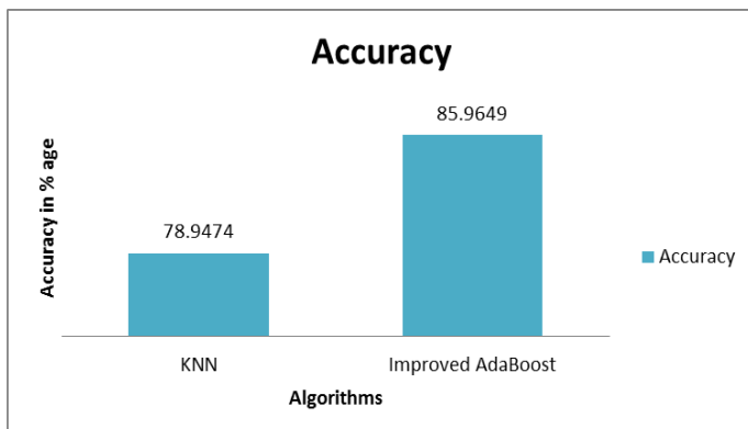
Figure 4: Accuracy Comparison
