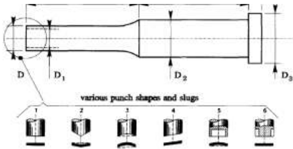
Fig. 1. Punch configuration with various punch shapes and slugs.
