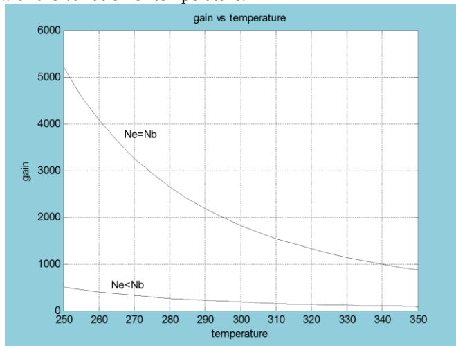
Figure 2: Gain vs Temperature for the designed heterojunction (with N_e < N_b and N_e = N_b )
