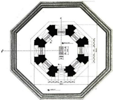
Sketch 15 Typical Plan of Mata Chamber
