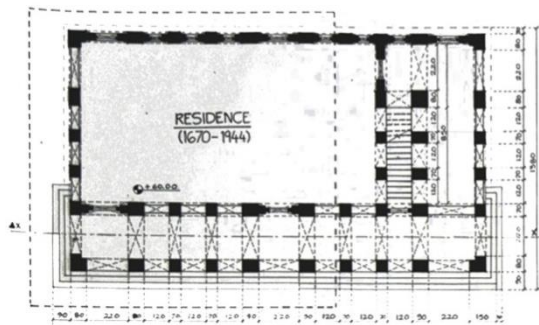
Sketch 6 First Floor Plan of Museum Source: Author
