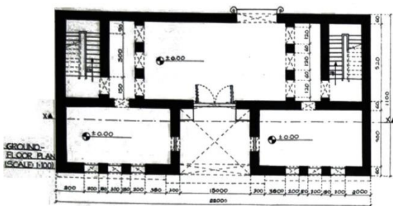
Sketch 5 Floor Plan of Elephant Gate Source: Author
