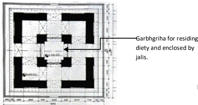
Sketch 8 Ground Floor Plan of Langar Darbar Sahib
