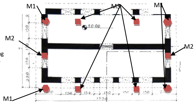
Sketch 10 Floor Plan of Darshini Dwar
