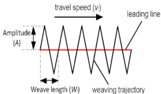
Fig. 9. Mechanical Weaving
