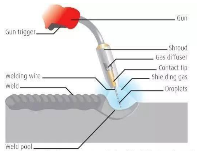
Fig. 1. Fusion Type Welding
