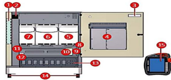
Fig. 7. Components of KRC4 Controller
