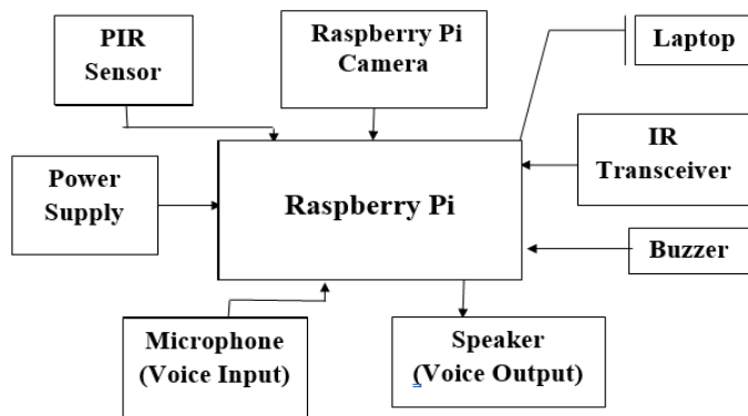
Figure 2: Block Diagram
