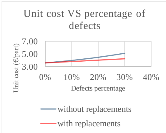
Figure 10: Effect of defects percentage on unit cost
