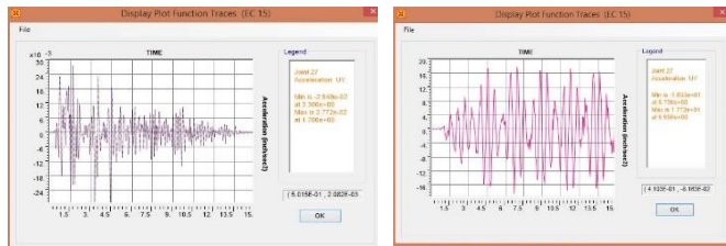
Figure 9. Mid-point acceleration vs time curve in Y axis (15 sec)
