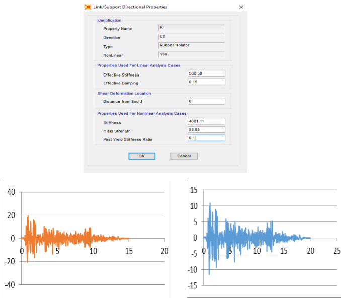
Figure 5. Acceleration vs. Time (Modified El Centro for 15 sec; 20 sec)
