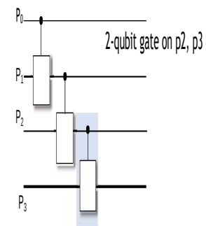
Figure 7d: Example program of IR
