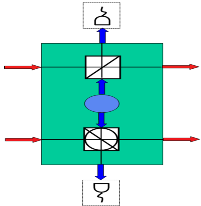
Figure 5: Linear Optical Quantum controlled NOT gate
