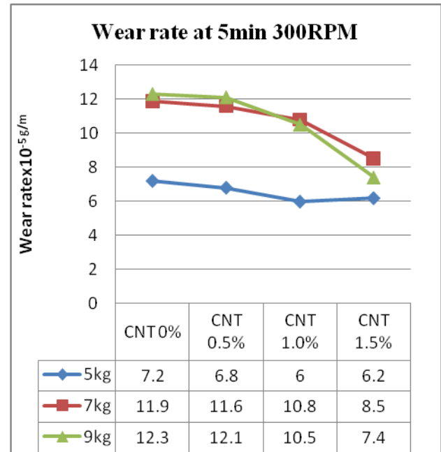
Graphic 7: % by weight CNT v / s wear rate (300 rpm, 5 min)
