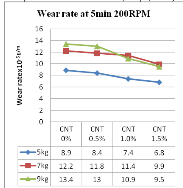
Graphic 4: % by weight CNT v / s wear rate (200 rpm, 5 min)
