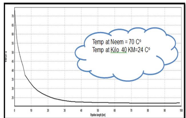
Figure (10) Pipeline temperature Profile for actual operation condition [16]
