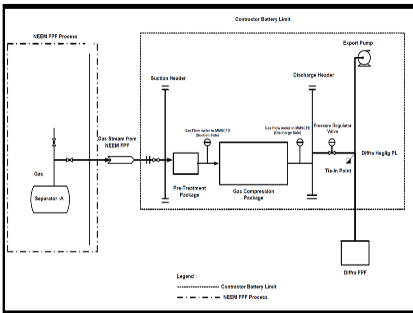
Figure (6) Crude Transferred to Diffra via Crude oil transfer pump
