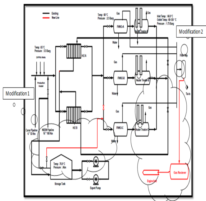
Figure (13) DIFFRA process Utilize Train –C to process the &separate the gas
