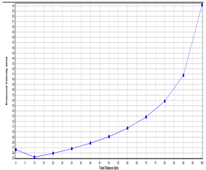
Figure 16 Erosional velocity[16]
