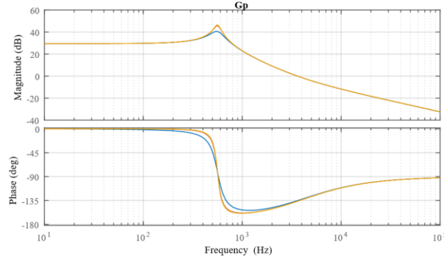
Fig. 11. Bode Plot of PID Colntrolled Buck Converter, Plant Gain
