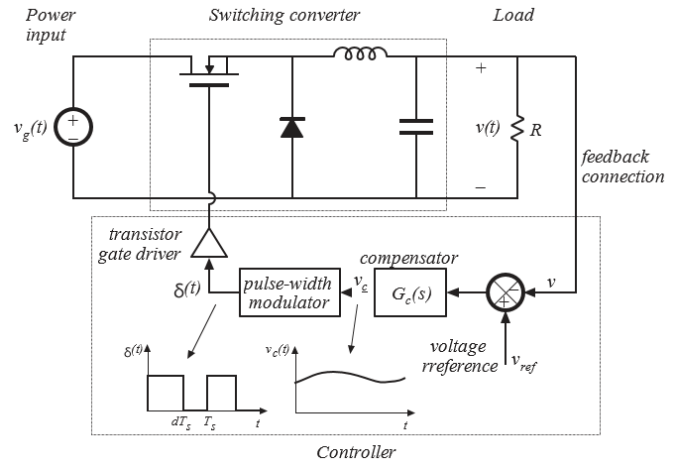
Fig. 2. Closed Loop control of a Buck Converter
