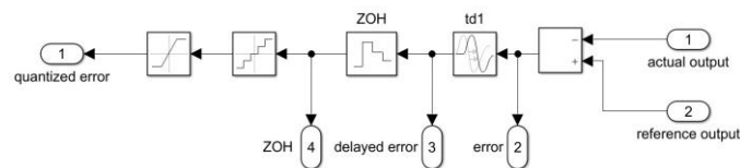
Fig. 20. Subsystem of Analog to digital Converter.
