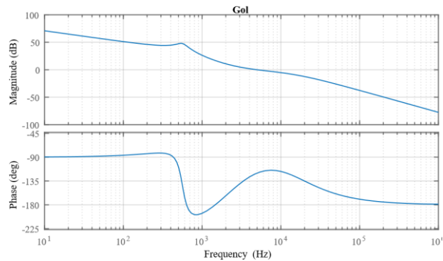
Fig. 13. Bode Plot of PID Colntrolled Buck Converter, Open-Loop Gain
