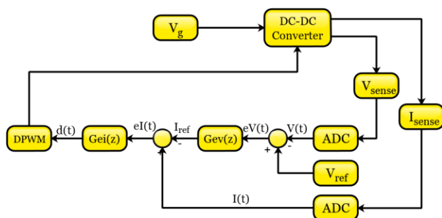
Fig. 7. Block Diagram Of Close-Loop
