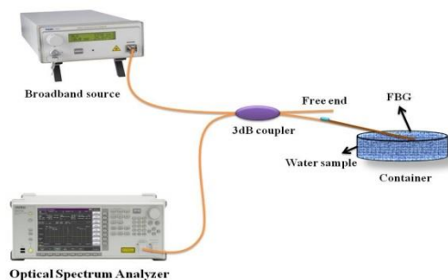
Fig.3. Experimental setup for the detection of lead in water
