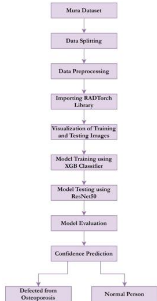
Figure 3 Proposed Methodology
