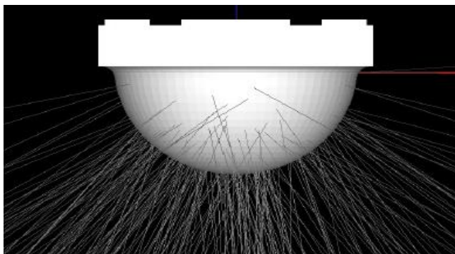
Fig.2: Tracing the LED rays by light distribution in space according to the calculation provided with an angle of 140 degrees.
