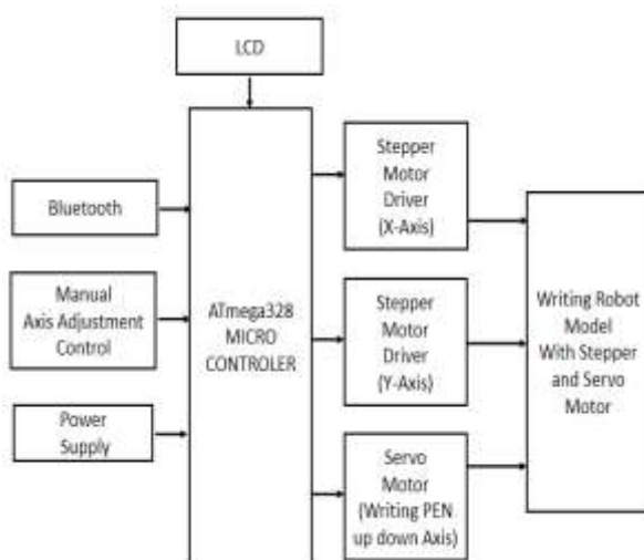
Fig. 3. Architecture diagram
