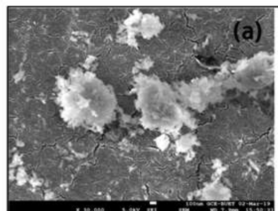
Morphological analysis of Synthesized nano urea by SEM
