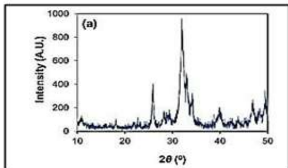
XRD Results of Hybrid Nano Fertilizer
