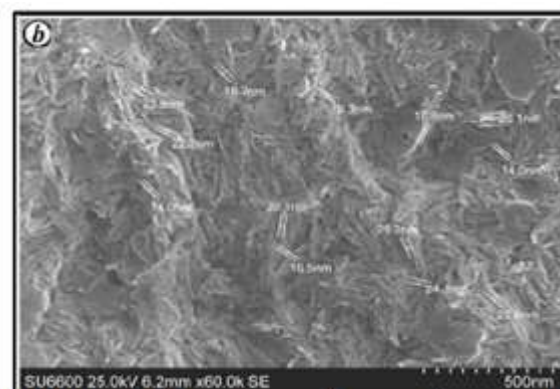
Morphological analysis of urea modified hydro xyapatite nano particles by SEM
