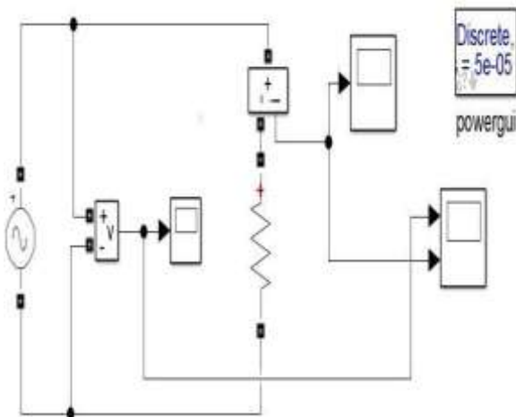
Fig. 10. Matlab model of pure resistive circuit
