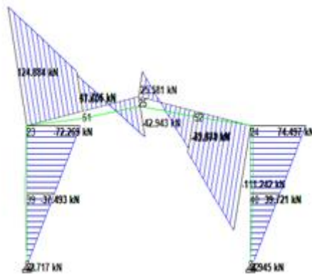
Fig 18. Shear Force diagram for intermediate frame for model PEB1
