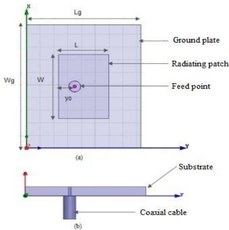
Fig. 1. Geometry of coaxial feed microstrip patch antenna [15] (a) Top view (b) side view
