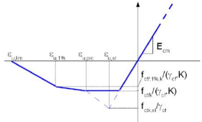
Figure 8 Stress - Strain Curve of Tensile Force
