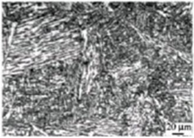
Fig.4.Welding microstructure map[11]
