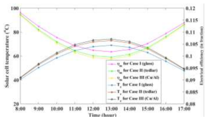
Fig. 5. Hourly variation of solar cell temperature and electrical efficiency
