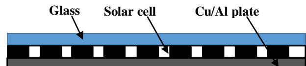
Fig. 1(c). Cut sectional view of opaque PV collector
