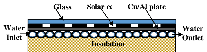
Fig.1d. Cut sectional view of Cu/Al base PVT water collector
