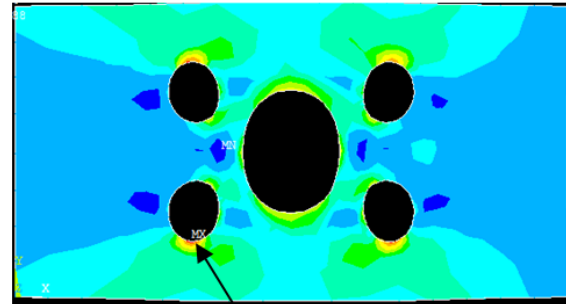
Maximum stress location
