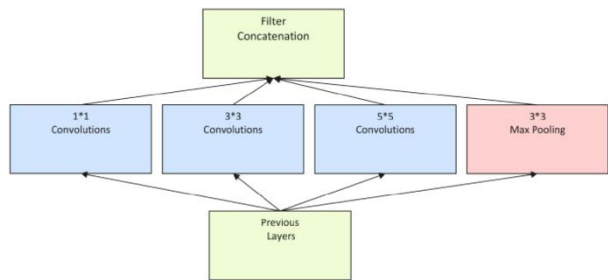
Fig 13: Architecture of Inception model [16]
