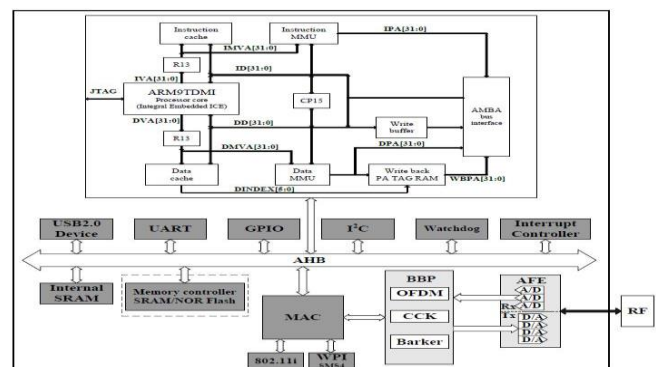
Fig1. Architecture of Wi-Fi chip (HED05W01SA)
