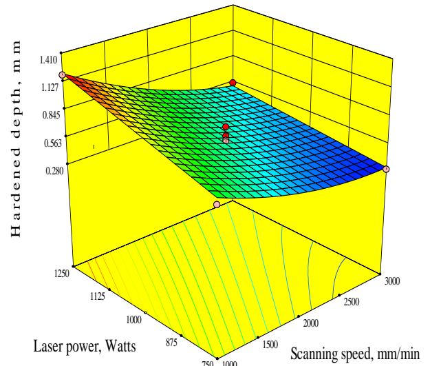
Figure 12. 3Dgraph shows the effect of LP and SS on the hardened depth
