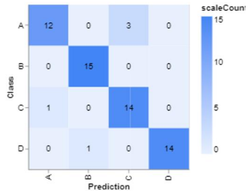
Fig. 12. Confusion Matrix
