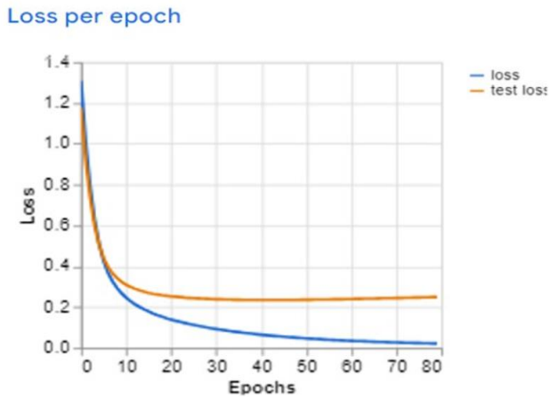
Fig. 10. Loss graph
