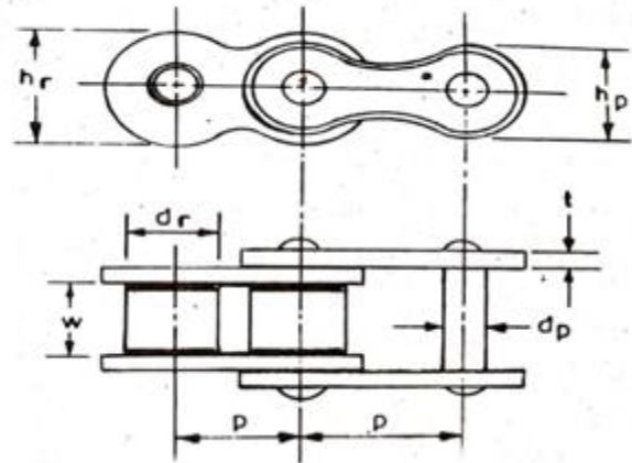
Fig.3: Chain linkages
