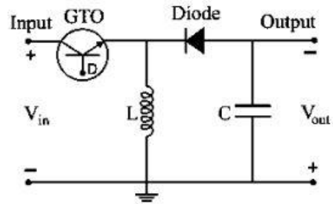
Figure 4: Buck-Boost topology
