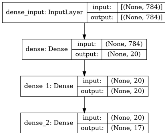
Fig 1. Dense Model Summary
