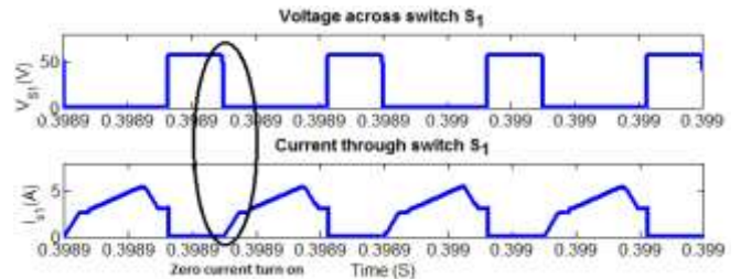
Fig .8. Zero current turn on of switch S_1
