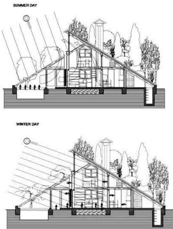
Fig. 2. Shading Measurements
