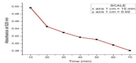
Fig: 4.3.1 Bromothymol Blue Assay for extraction procedure-5
