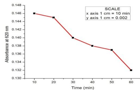
Fig: 4.3.1c) Bromothymol blue assay for extraction procedure-3
