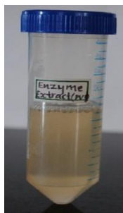
Fig: 4.2.5.1 Enzyme extract obtained using PVPP
