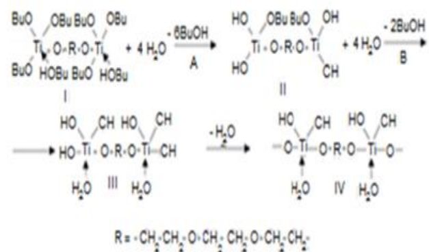
Fig.1: The adduct film-forming process using TBT TEG (I)
