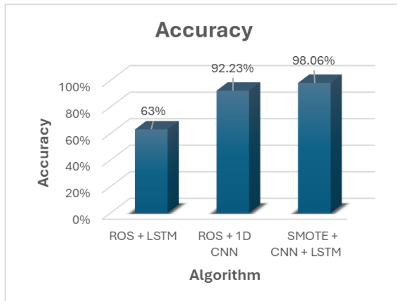
Fig. 7. Comparative Analysis of Classification Accuracy Across Balanced Algorithms
