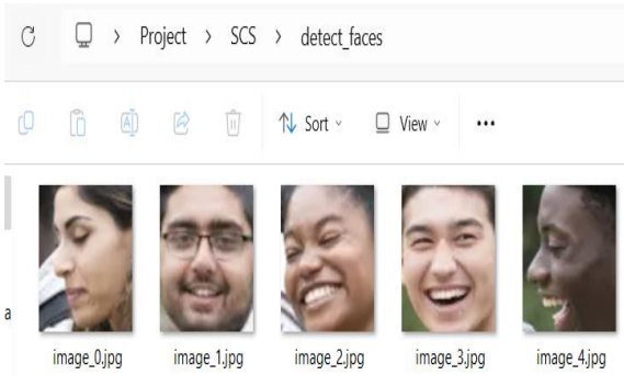
Fig 12: Cropped Faces
