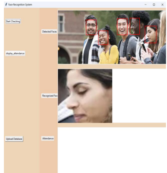
Fig 16: Recognized Image
