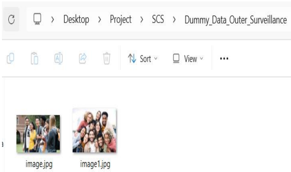
Fig 8: 'Dummy_Data_Outer_Surveillance' folder
