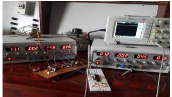
Fig. 25. Experimental setup for new transformerless buck-boost converter
