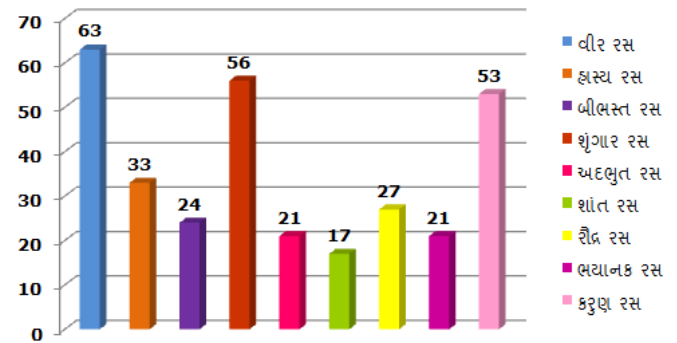
Figure 1 'Kavan' Dataset
