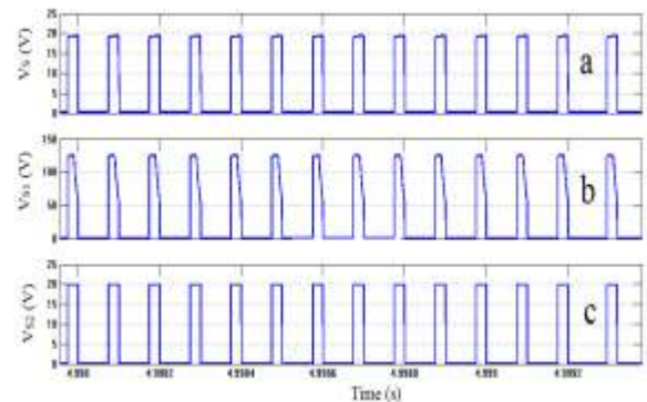
Fig. 10: (a) Voltage Stress across switch S (b) Voltage Stress across switch S_1 (c) Voltage Stress across switch S_2
