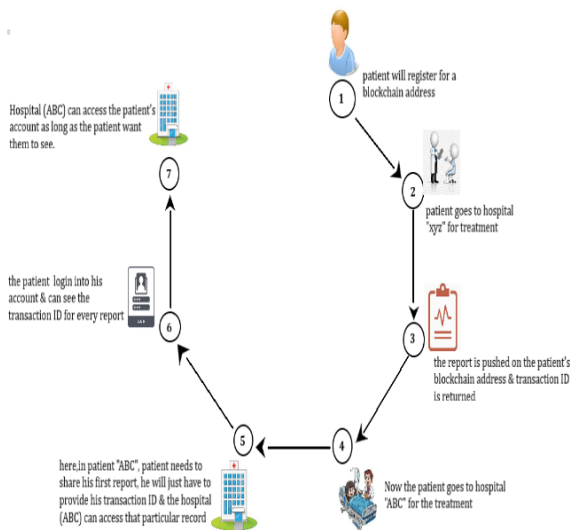
Figure 1: Architecture Diagram
