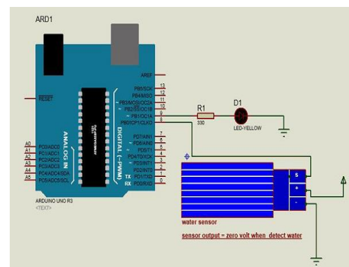
Fig 10: Water sensor
