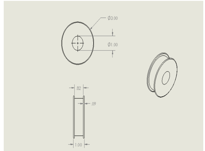
Fig 16: Dimensions of Pulley
