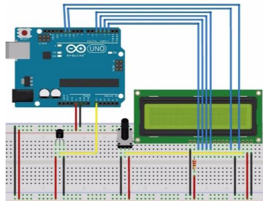
Fig 12: Circuit diagram
