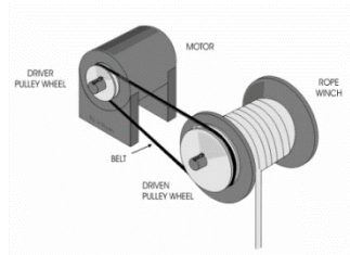
Fig 6: Pulley and Rope mechanism
