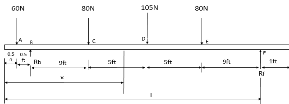
Fig 27: Deflection
