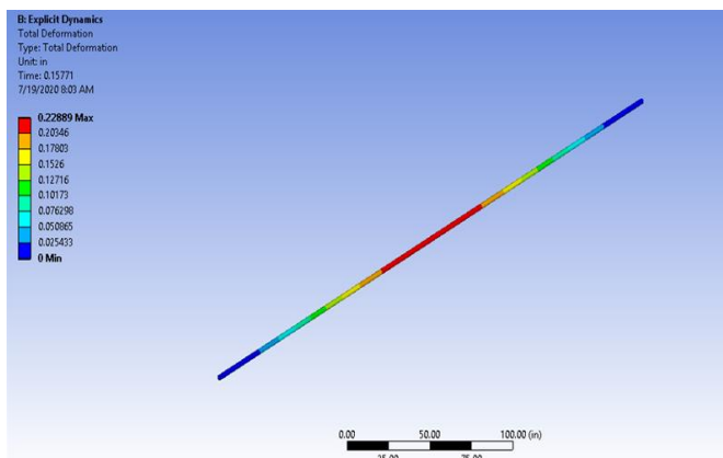
Fig 28: Total Deformation of Shaft
