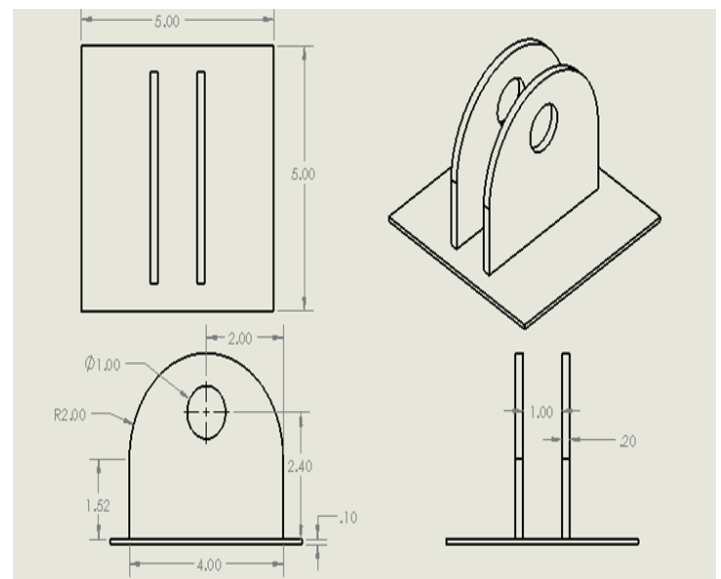
Fig 17: Dimensions of Pulley Support
