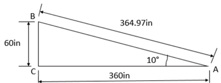
Fig 22: The slope between drum and pulley
