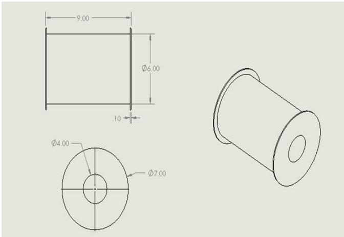
Fig 18: Dimensions of Drum
