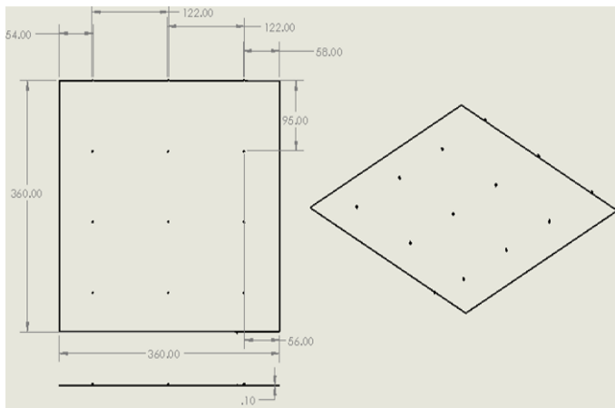
Fig 15: Dimension of Curtain
