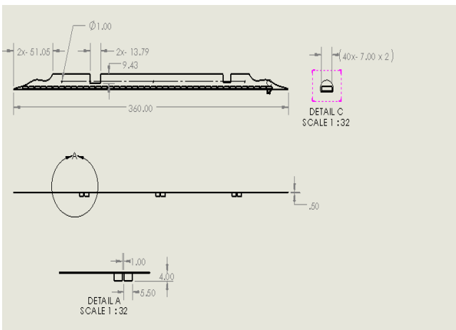
Fig 19: Dimensions for Drive Unit
