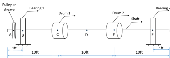
Fig 26: Shaft
